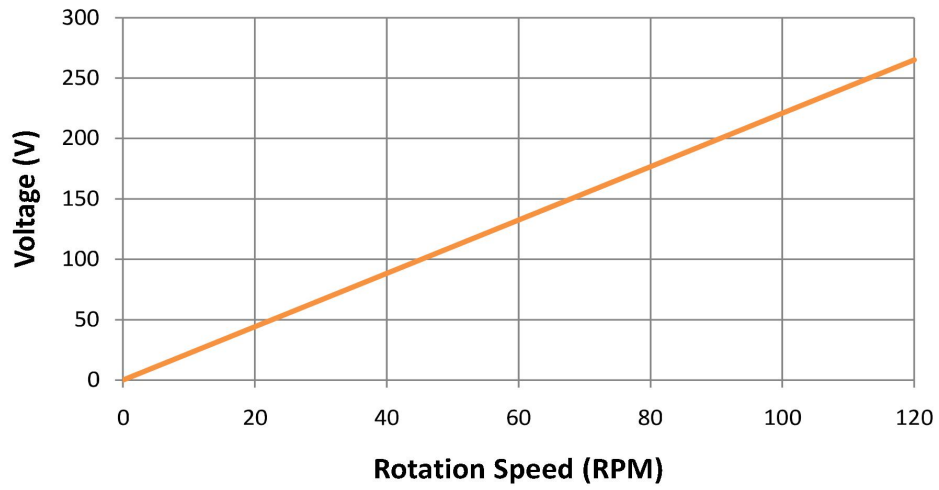
Speed-Load Voltage Curve
